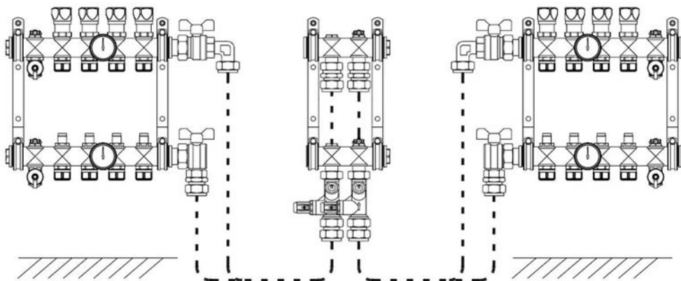
Example of installation with Thermotech Group Manifold 1"
